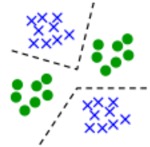
Multi-modal
